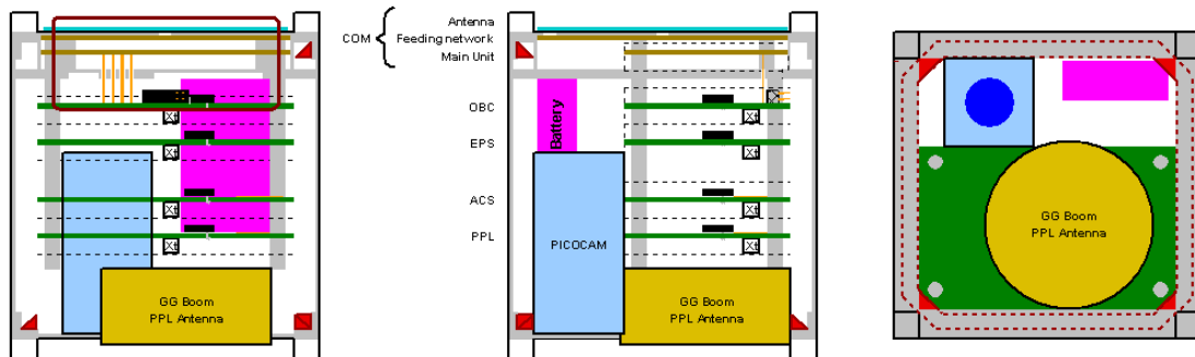
Figure 6. The configuration of DTUsat. The brown and green slabs indicate printed circuit boards seen edge on. The red triangles denote the electromagnetic coils for the attitude control.
