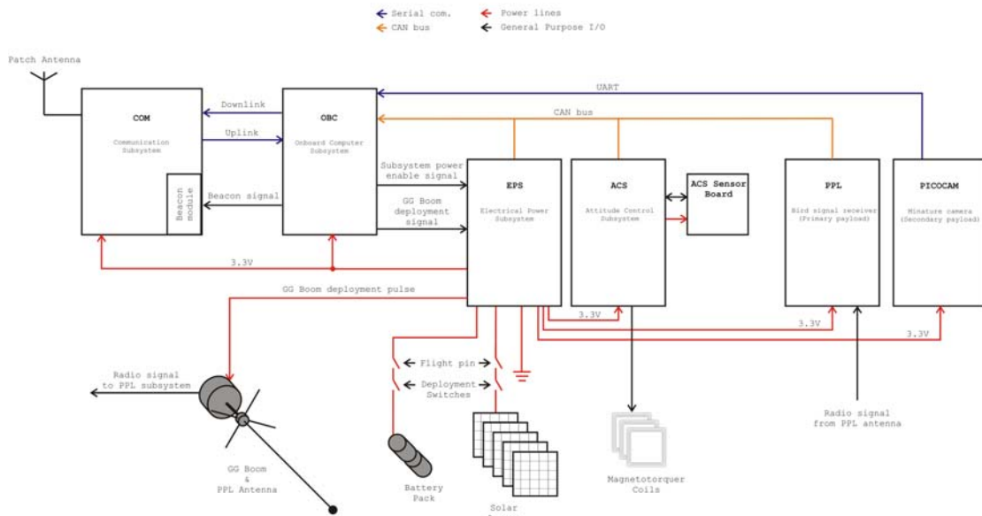
Figure 5. The DTUsat topology, the subsystems, and their interconnections.
